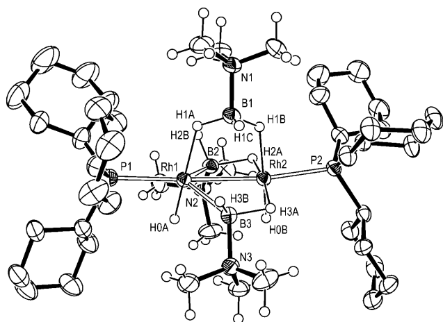
Figure 1. Solid-state structure of \mathbf{2}\text{-Cy}^{2+} . Thermal ellipsoids set at 50 % probability; phosphine H-atoms omitted for clarity. Selected bond lengths [Å] and angles [°]: Rh1–Rh2 2.6292(4), Rh1–P1 2.4025(10), Rh2–P2 2.3559(10), Rh1–B1 2.747(5), Rh1–B2 2.086(4), Rh1–B3 2.086(4), Rh2–B1 2.757(5), Rh2–B2 2.217(4), Rh2–B3 2.233(4), Rh1–H0A 1.46(4), Rh2–H0B 1.50(4), Rh1–H1A 1.88(5), Rh2–H1B 1.86(5), B1–H1A 1.21(5), B1–H1B 1.22(5), B1–H1C 1.15(5), B2–H2A 1.43(5), B2–H2B 1.12(5), B3–H3A 1.34(5), B3–H3B 1.10(5), P1–Rh1–Rh2 176.55(3), Rh1–Rh2–P2 171.91(3).
